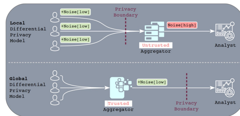
Figure 2.1: Depending on the site where noise is added, approaches to differential privacy can be categorized into local and global models.
