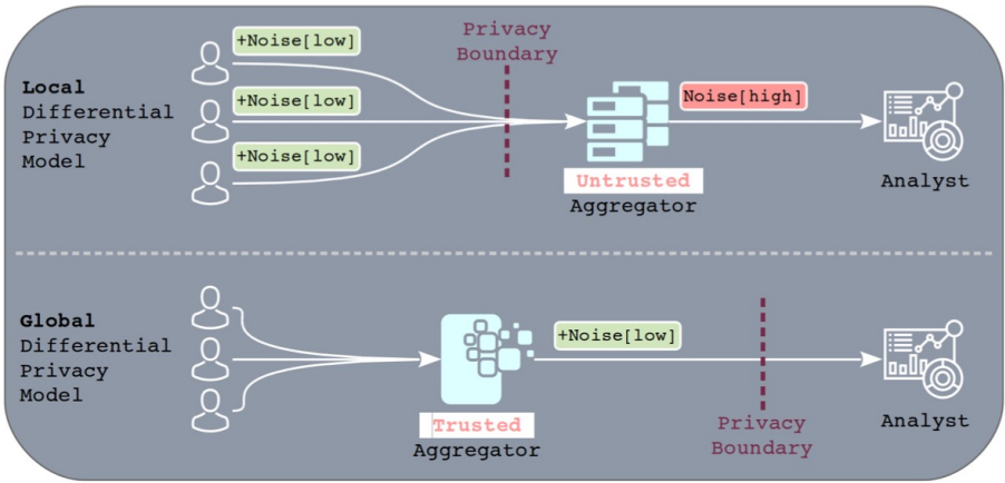
Figure 2.1: Depending on the site where noise is added, approaches to differential privacy can be categorized into local and global models.
